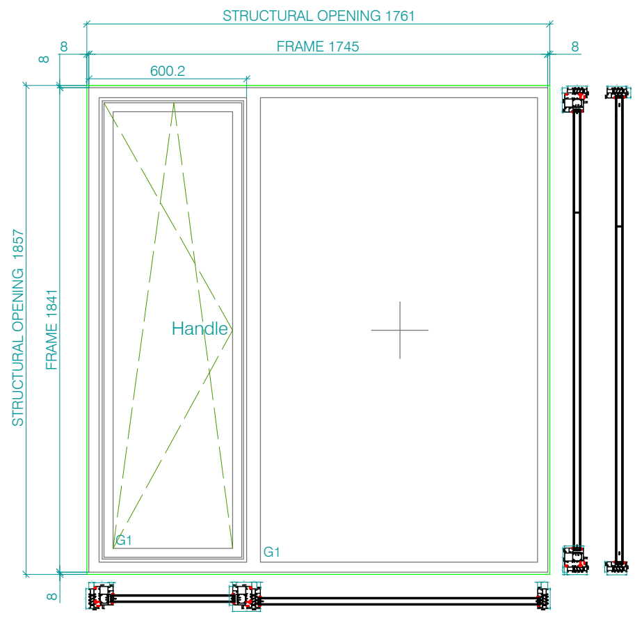
REYNAERS SL38 TILT & TURN + FIXED VIEWED FROM THE OUTSIDE QUANTITY = 1 LOCATION:
