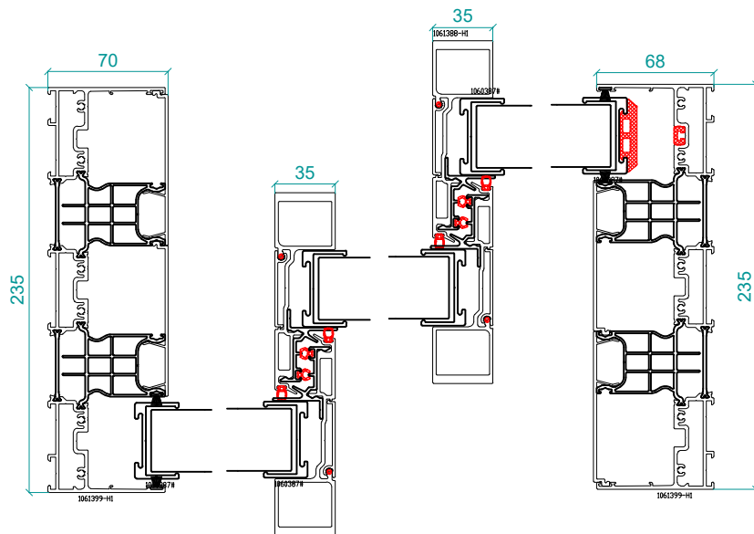
Hi-Finity Triple Track VIEWED FROM THE OUTSIDE Quantity = 1
